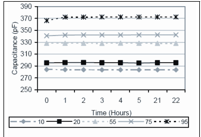
FIGURE 7: SHORT-TERM STABILITY
