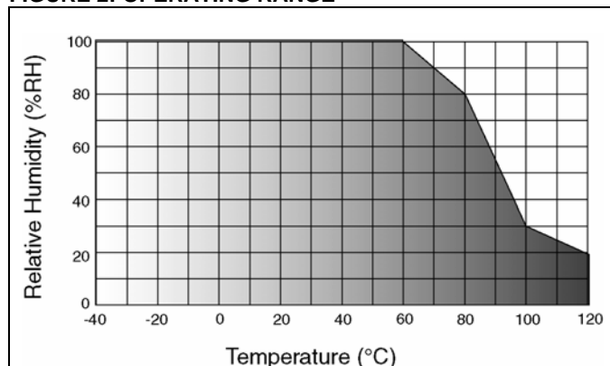
FIGURE 2: OPERATING RANGE
