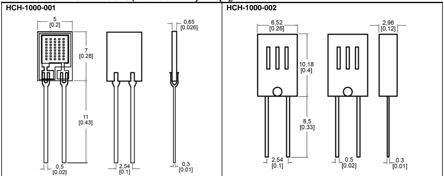
FIGURE 8: MOUNTING DIMENSIONS (For reference only: mm/[in])
