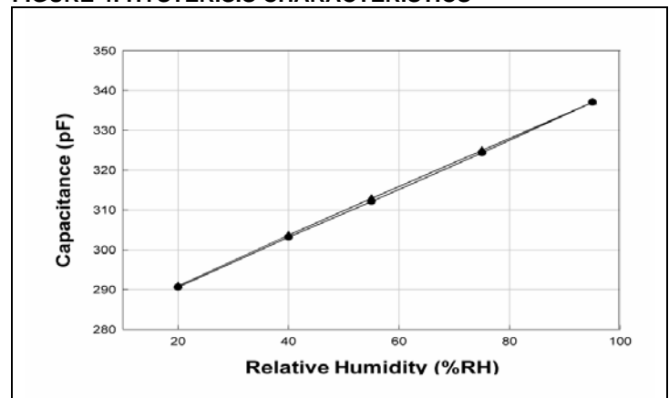
FIGURE 4: HYSTERISIS CHARACTERISTICS
